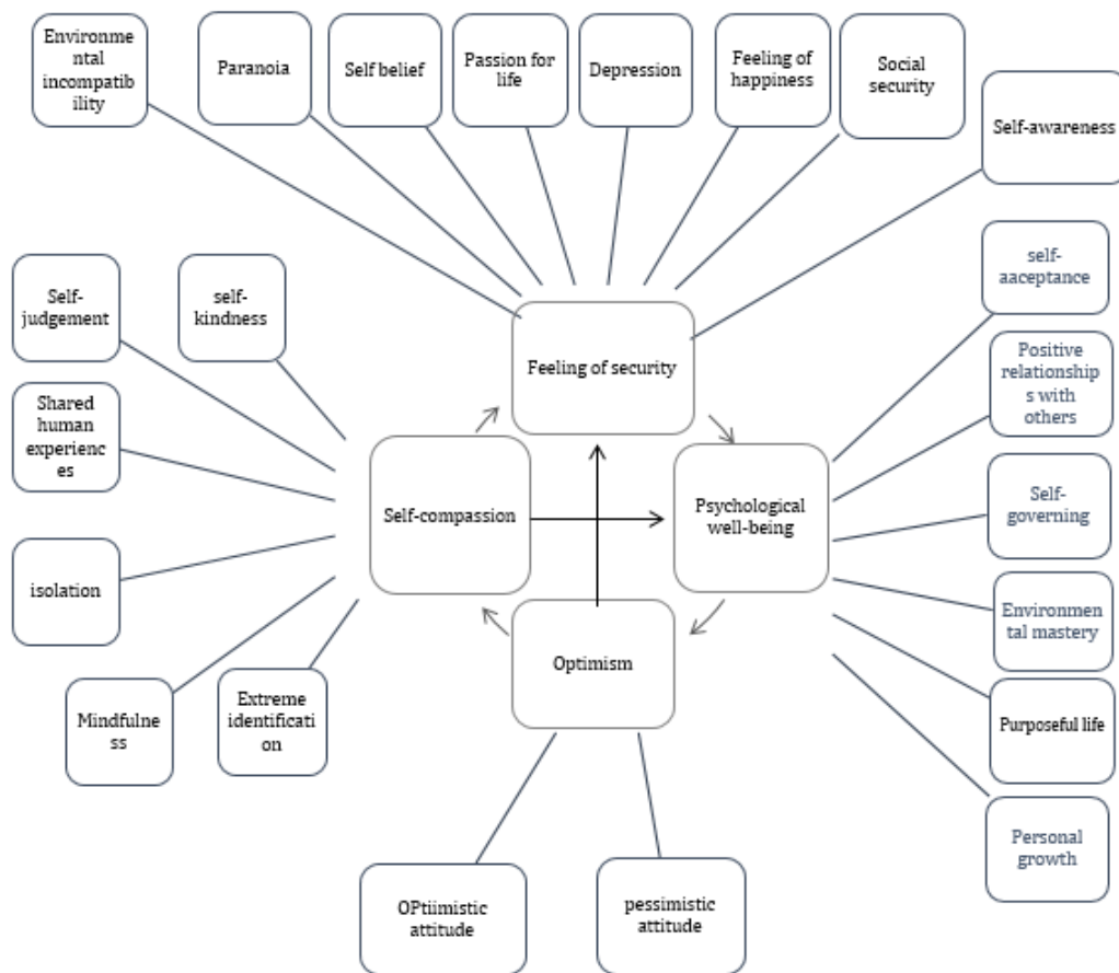
Figure 1. Structural equation modeling fit chart according to the conceptual model and coefficients of relationship between variables
