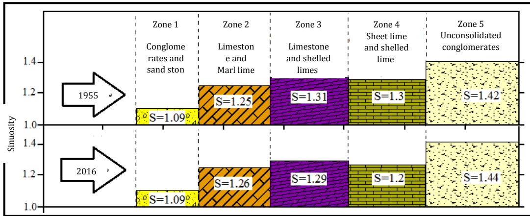
Figure 4) sinuosity values in different zones of Khorram Abad river
