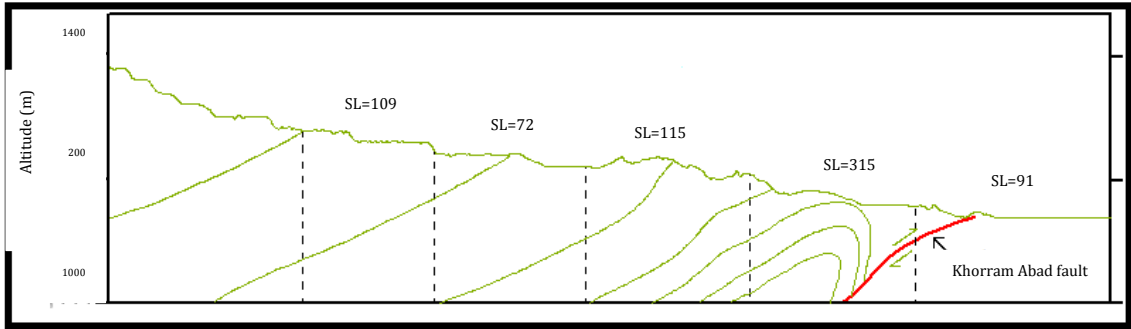
Graph 1) SL value in different zones of Khorram Abad river
