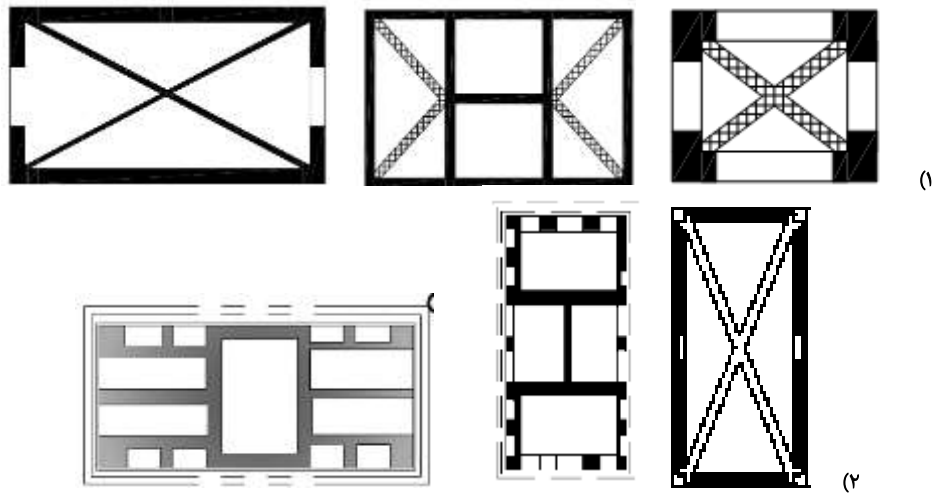
Figure 7) rectangular windcatchers
