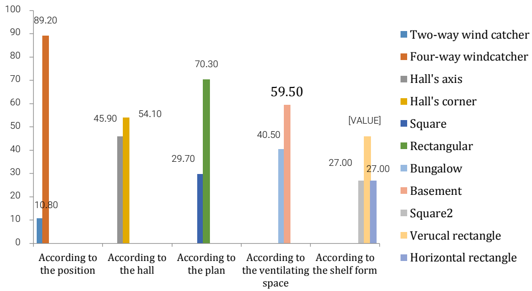
Figure 10) The Typology of all types of wind catchers in Semnan (percentage)
