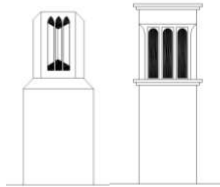
b) the wind catchers with vertical rectangular shelves
