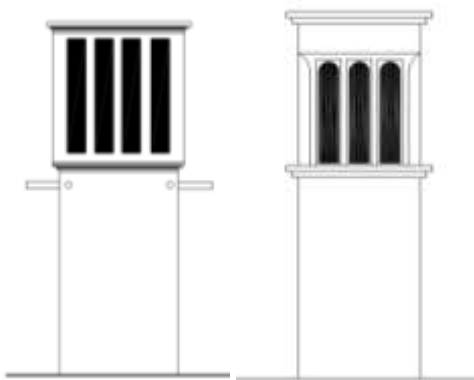
Figure 9) a) the wind catchers with square shelves
