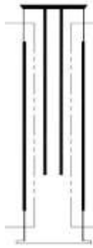
Figure 8) a) Seyed Kazem house wind catcher cross-sectional area (Type D1)
