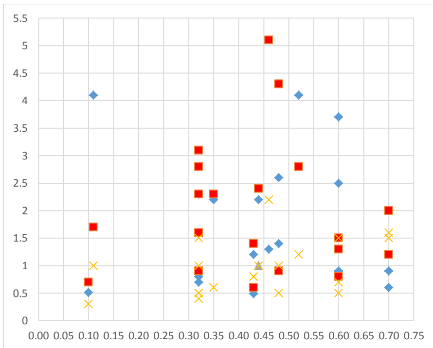
Graph 2) maximum water flow in sub-basins caused by different rainfalls
