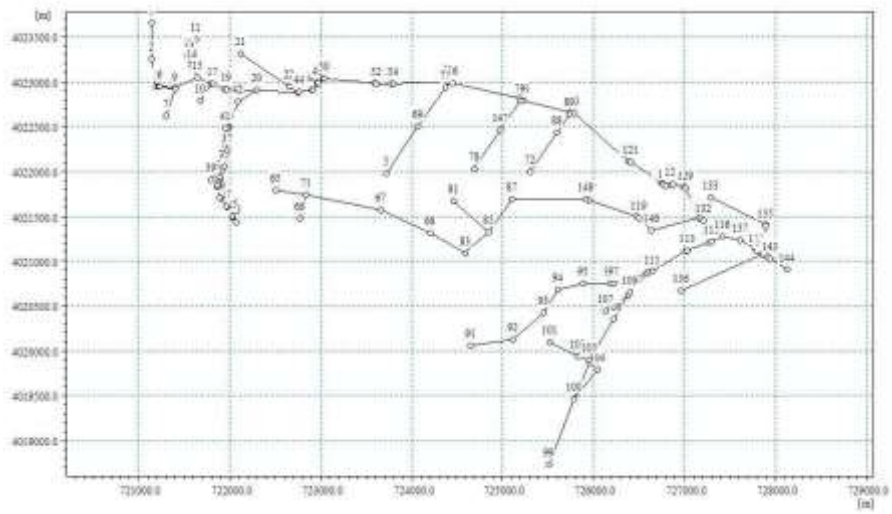
Figure 3) sub-basins discharging in inlet nodes of the run-off transfer system in water and electricity neighborhood in 2020
